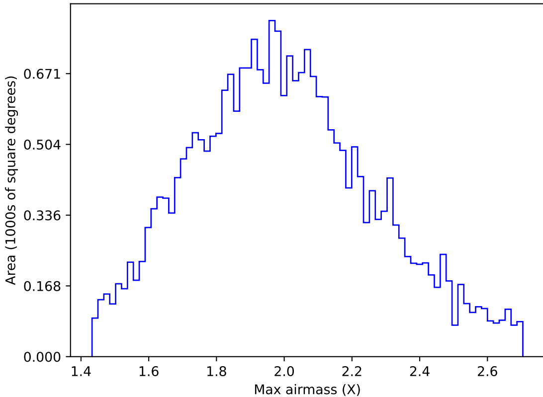
early_u_fpextra2.0_v3.4_10yrs All sky g band: Max airmass
