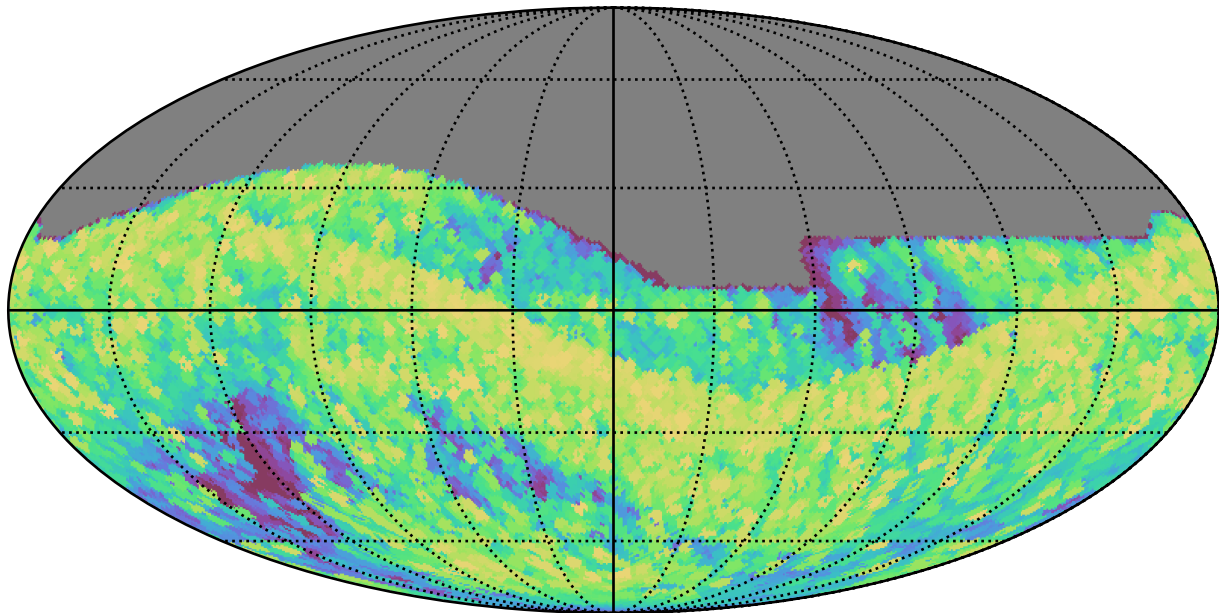
early_u_fpextra2.0_v3.4_10yrs All sky all bands: Max airmass
