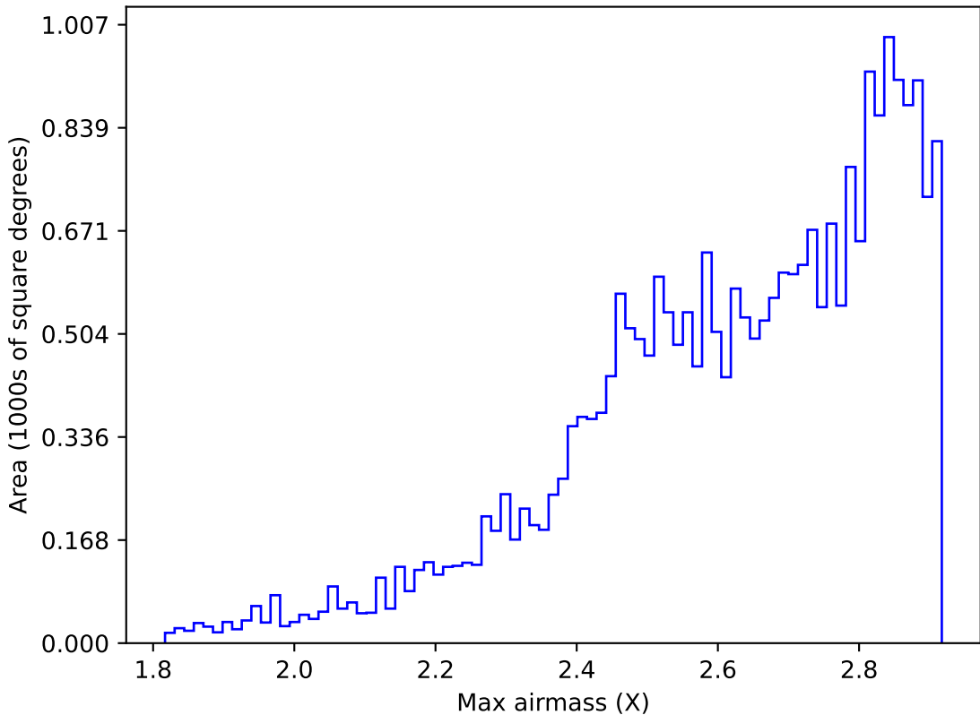
early_u_fpextra2.0_v3.4_10yrs All sky all bands: Max airmass
