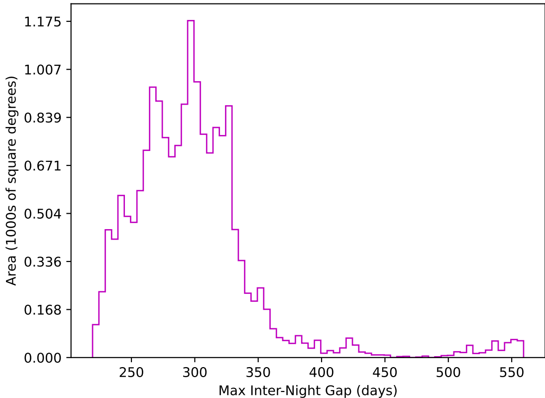
early_u_fpextra2.0_v3.4_10yrs WFD z band: Max Inter-Night Gap
