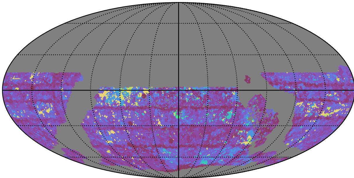
early_u_fpextra2.0_v3.4_10yrs WFD y band: Max Inter-Night Gap
