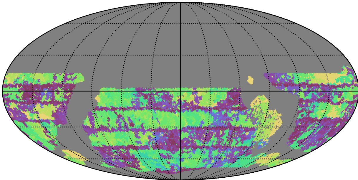
early_u_fpextra2.0_v3.4_10yrs WFD u band: Max Inter-Night Gap
