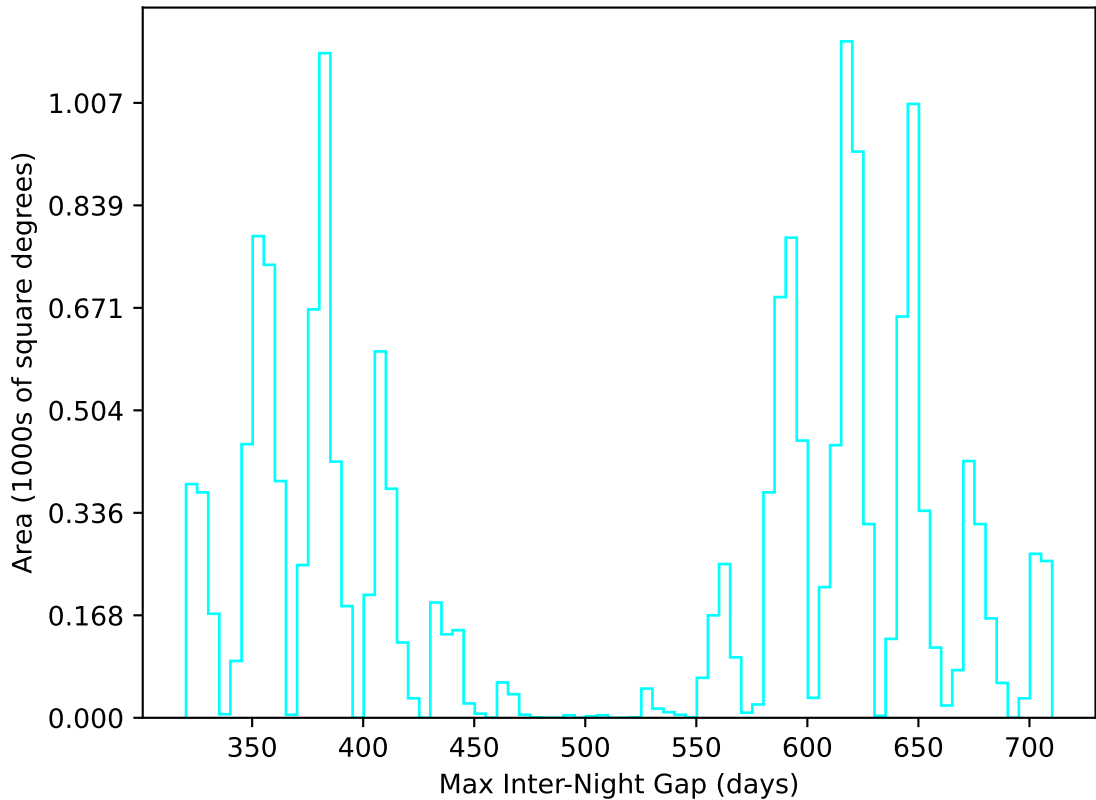
early_u_fpextra2.0_v3.4_10yrs WFD u band: Max Inter-Night Gap
