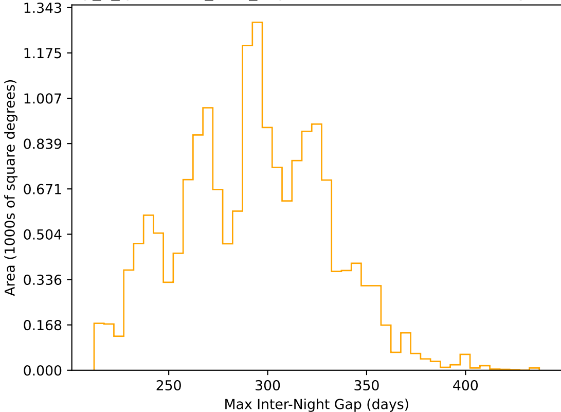
early_u_fpextra2.0_v3.4_10yrs WFD r band: Max Inter-Night Gap
