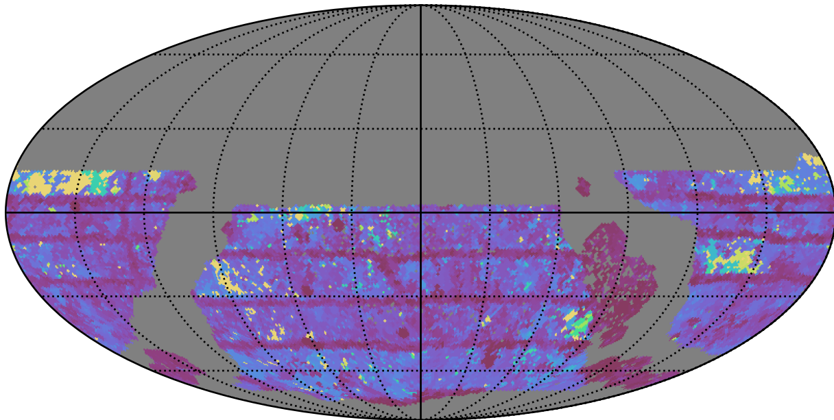
early_u_fpextra2.0_v3.4_10yrs WFD i band: Max Inter-Night Gap
