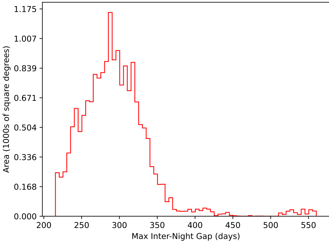
early_u_fpextra2.0_v3.4_10yrs WFD i band: Max Inter-Night Gap
