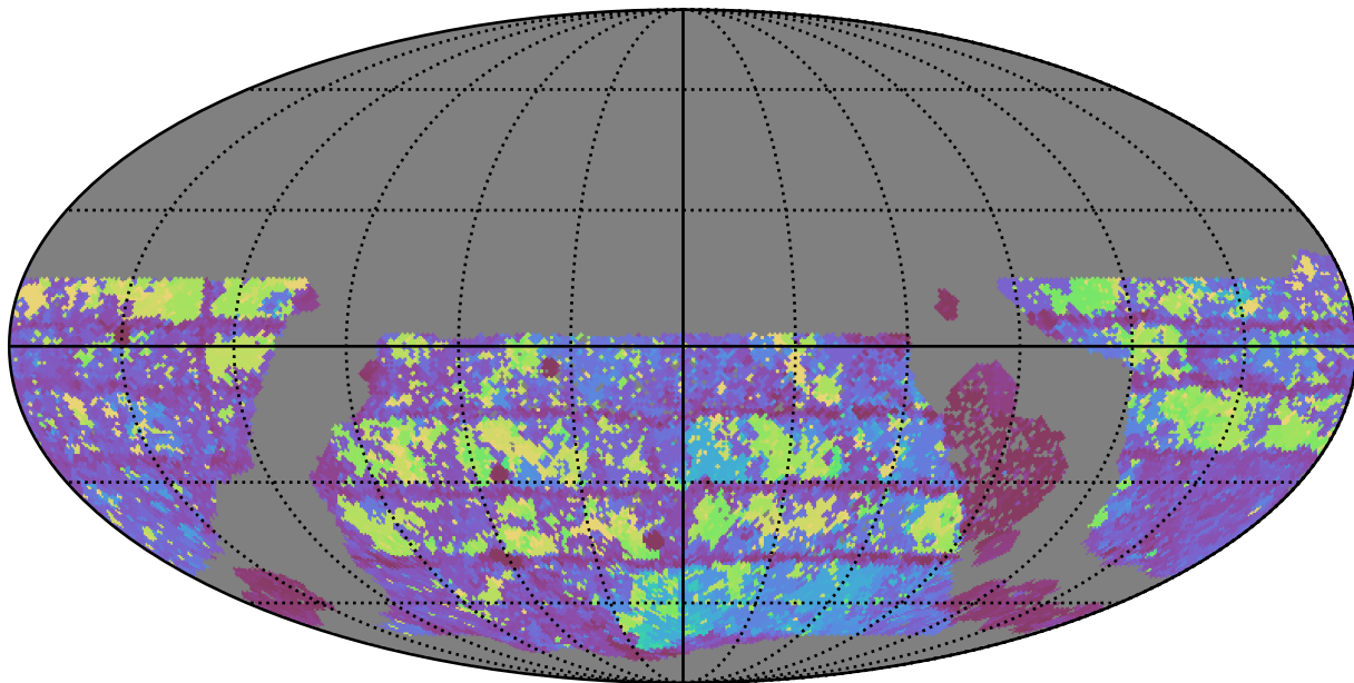
early_u_fpextra2.0_v3.4_10yrs WFD g band: Max Inter-Night Gap
