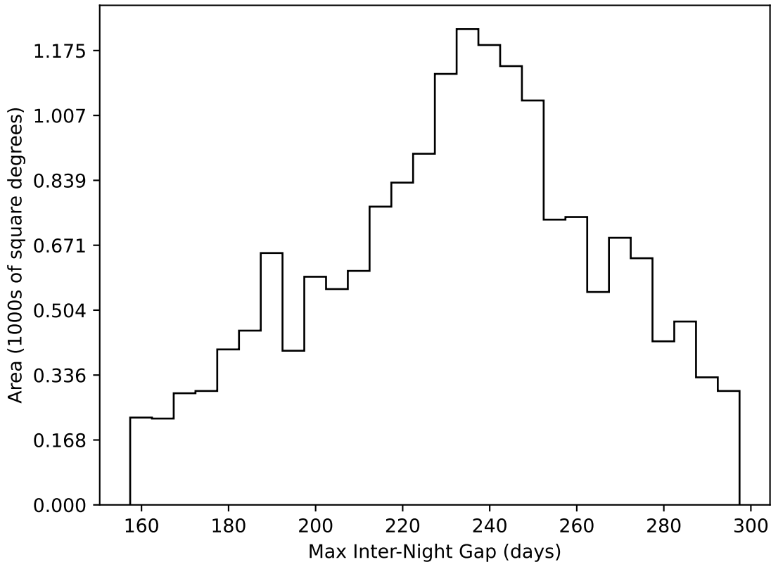
early_u_fpextra2.0_v3.4_10yrs WFD all bands: Max Inter-Night Gap
