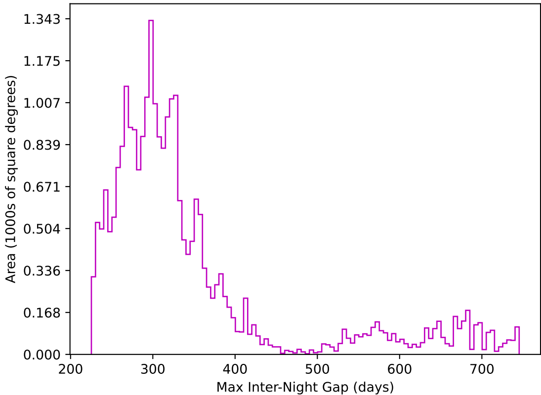
early_u_fpextra2.0_v3.4_10yrs All sky z band: Max Inter-Night Gap
