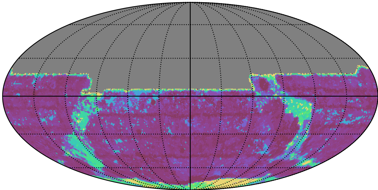
early_u_fpextra2.0_v3.4_10yrs All sky y band: Max Inter-Night Gap
