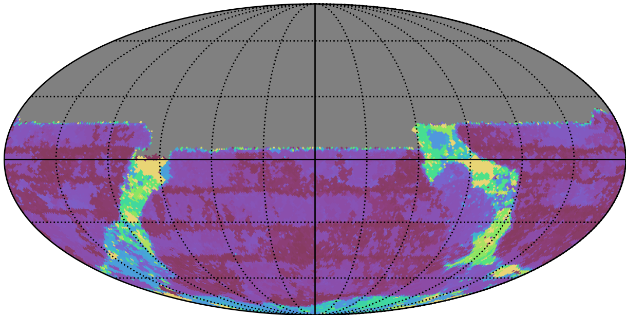
early_u_fpextra2.0_v3.4_10yrs All sky u band: Max Inter-Night Gap
