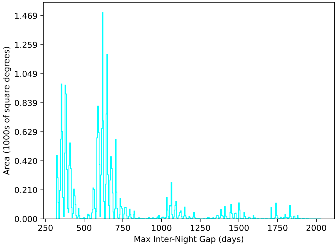
early_u_fpextra2.0_v3.4_10yrs All sky u band: Max Inter-Night Gap
