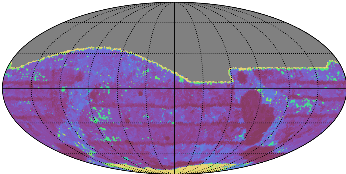
early_u_fpextra2.0_v3.4_10yrs All sky r band: Max Inter-Night Gap
