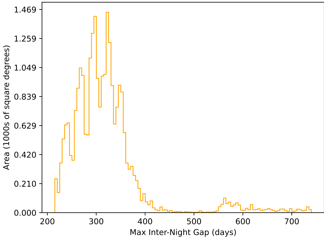
early_u_fpextra2.0_v3.4_10yrs All sky r band: Max Inter-Night Gap
