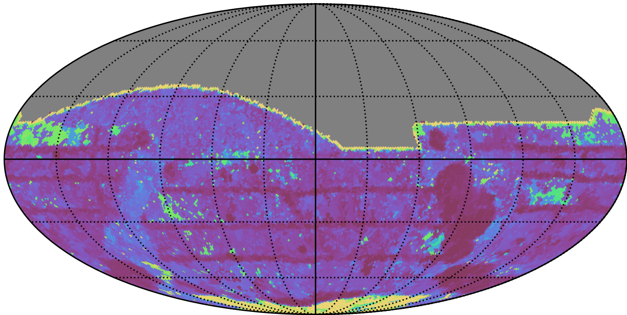
early_u_fpextra2.0_v3.4_10yrs All sky i band: Max Inter-Night Gap
