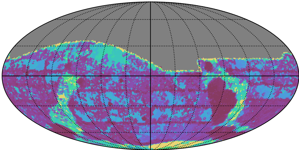
early_u_fpextra2.0_v3.4_10yrs All sky g band: Max Inter-Night Gap
