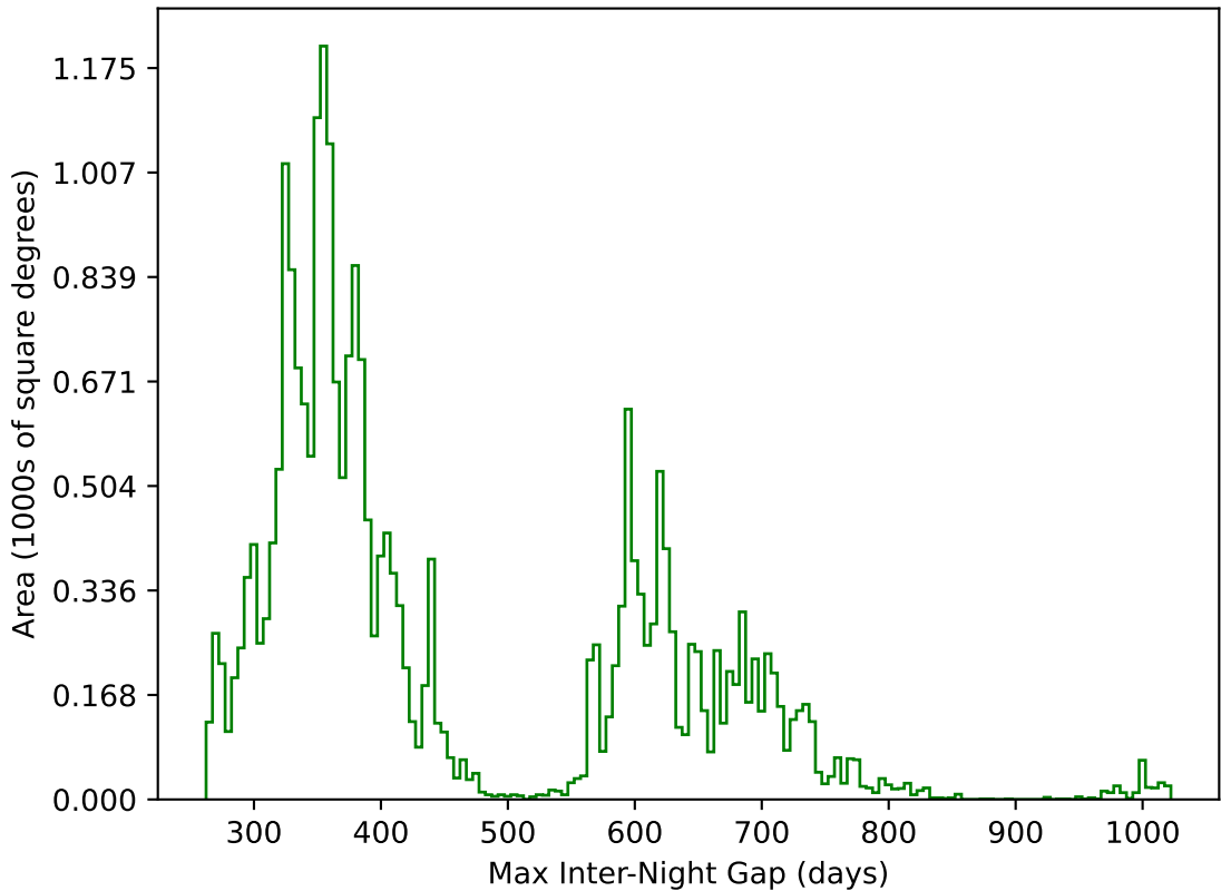
early_u_fpextra2.0_v3.4_10yrs All sky g band: Max Inter-Night Gap
