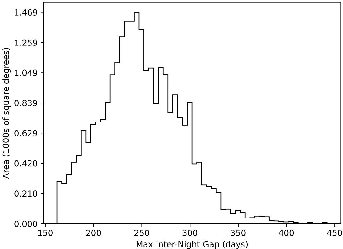
early_u_fpextra2.0_v3.4_10yrs All sky all bands: Max Inter-Night Gap
