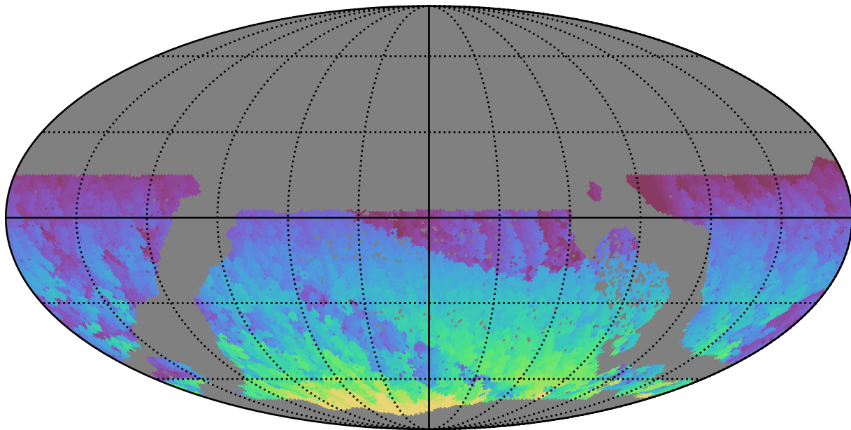
early_u_fpextra2.0_v3.4_10yrs WFD z band: Max HA
