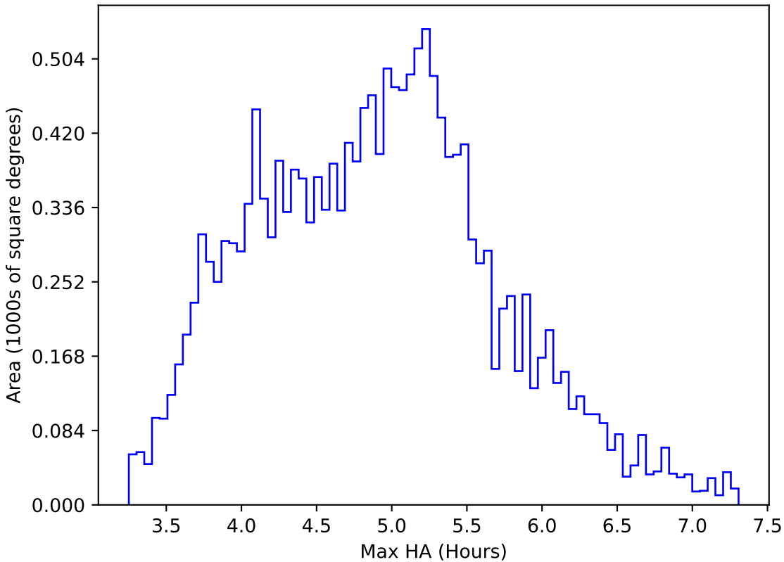
early_u_fpextra2.0_v3.4_10yrs WFD z band: Max HA
