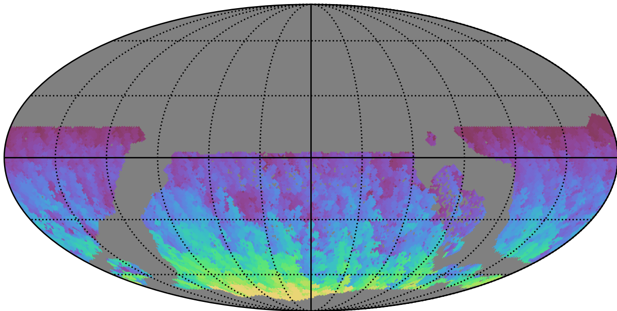
early_u_fpextra2.0_v3.4_10yrs WFD y band: Max HA
