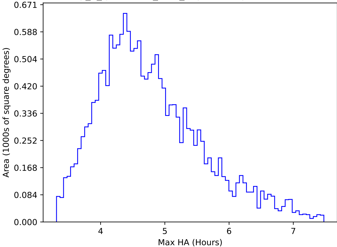
early_u_fpextra2.0_v3.4_10yrs WFD y band: Max HA
