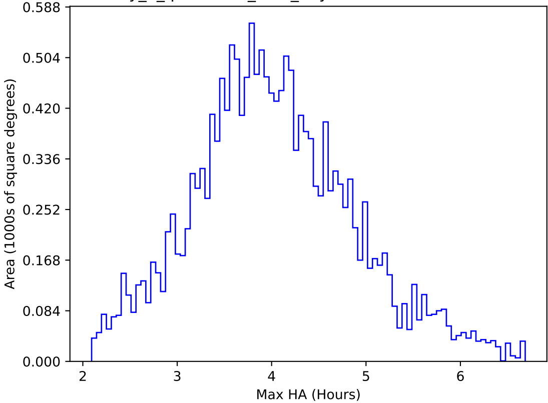
early_u_fpextra2.0_v3.4_10yrs WFD u band: Max HA
