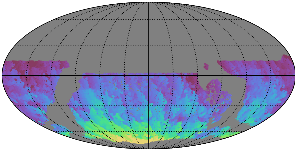
early_u_fpextra2.0_v3.4_10yrs WFD r band: Max HA
