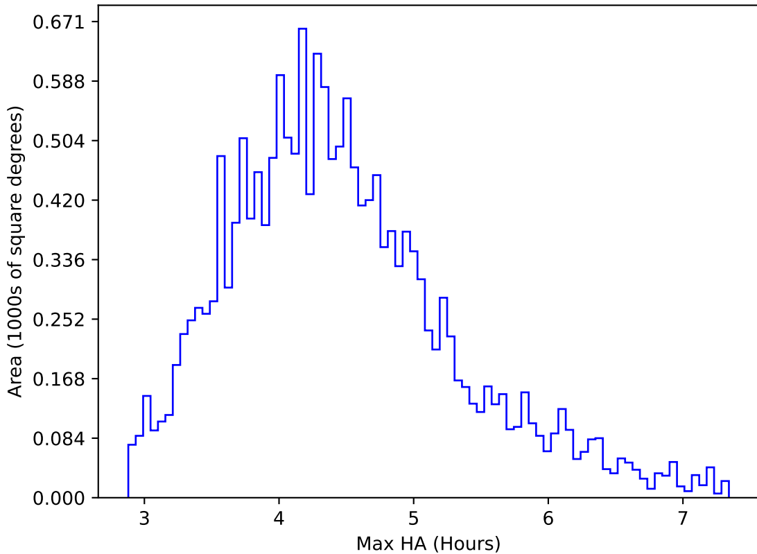
early_u_fpextra2.0_v3.4_10yrs WFD r band: Max HA
