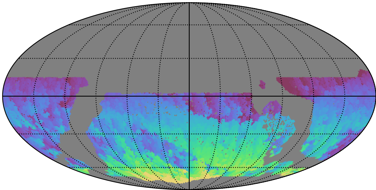
early_u_fpextra2.0_v3.4_10yrs WFD i band: Max HA
