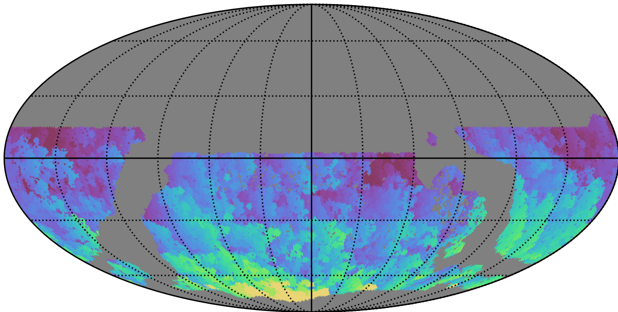
early_u_fpextra2.0_v3.4_10yrs WFD g band: Max HA
