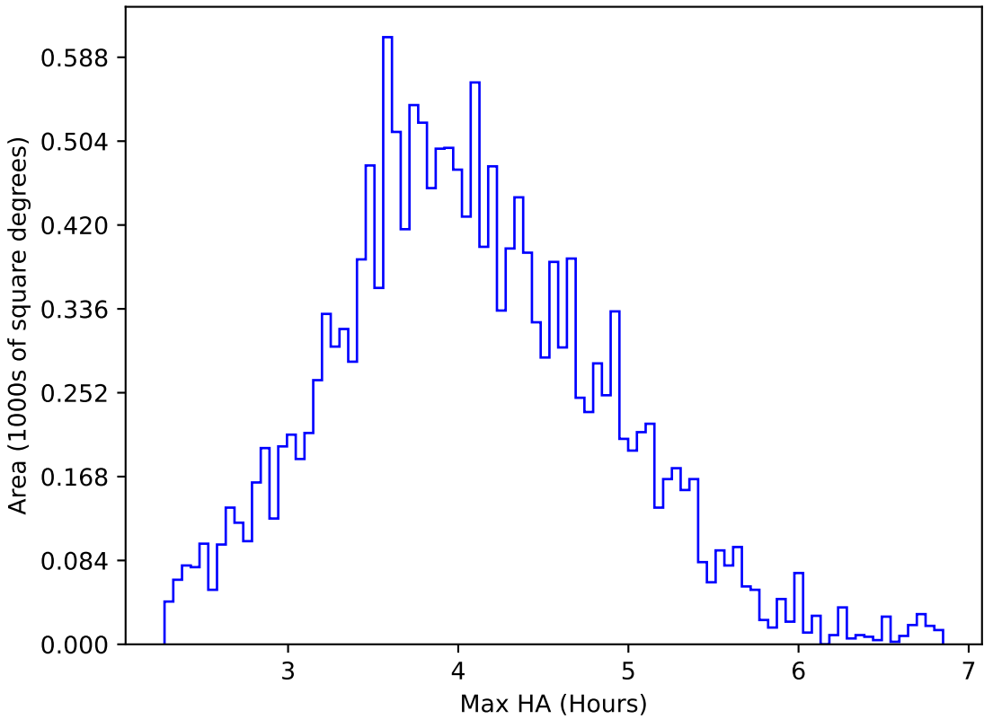
early_u_fpextra2.0_v3.4_10yrs WFD g band: Max HA
