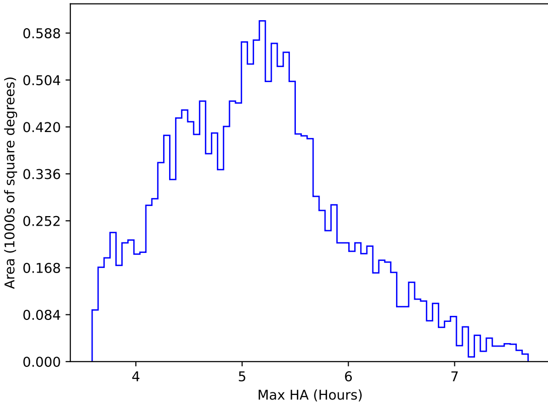
early_u_fpextra2.0_v3.4_10yrs WFD all bands: Max HA
