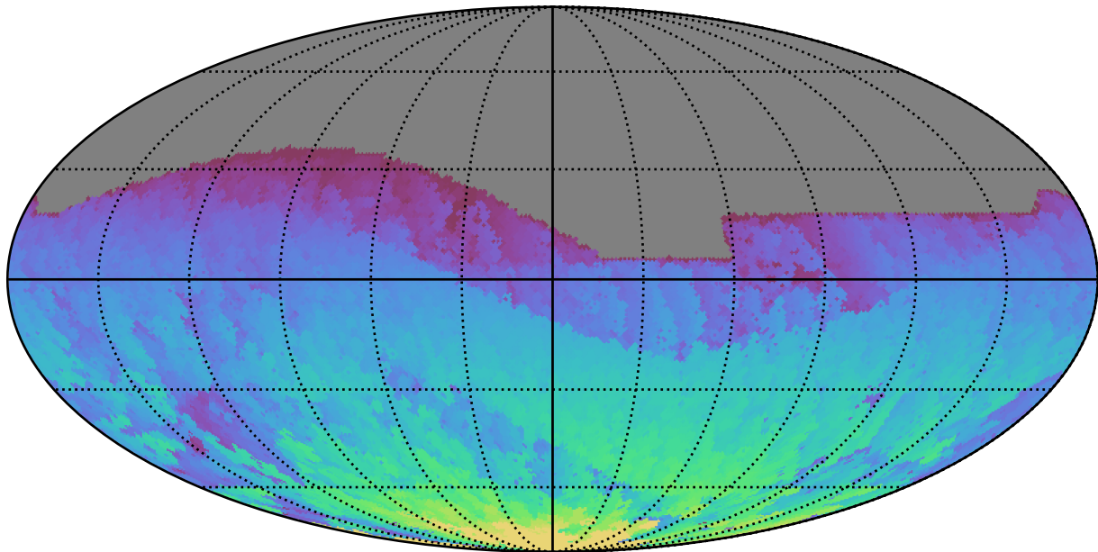
early_u_fpextra2.0_v3.4_10yrs All sky z band: Max HA
