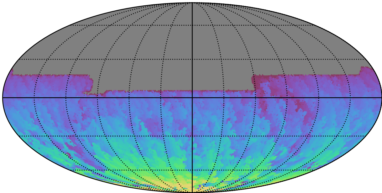
early_u_fpextra2.0_v3.4_10yrs All sky y band: Max HA
