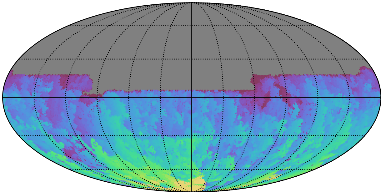
early_u_fpextra2.0_v3.4_10yrs All sky u band: Max HA
