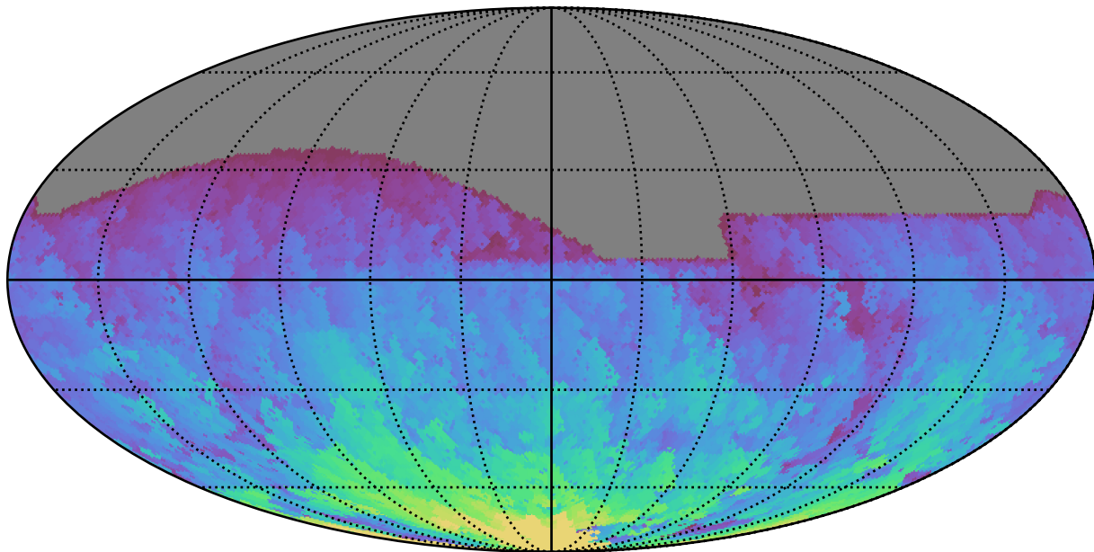
early_u_fpextra2.0_v3.4_10yrs All sky r band: Max HA
