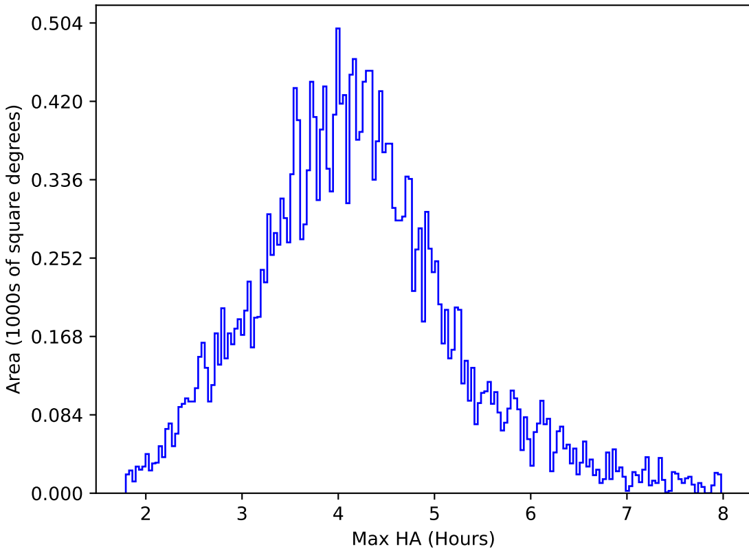
early_u_fpextra2.0_v3.4_10yrs All sky r band: Max HA
