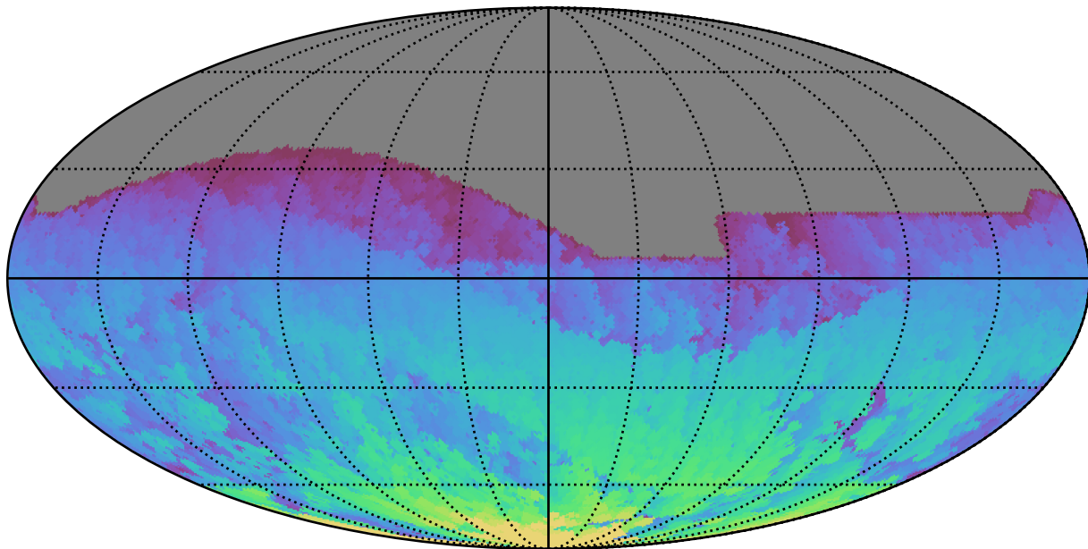
early_u_fpextra2.0_v3.4_10yrs All sky i band: Max HA
