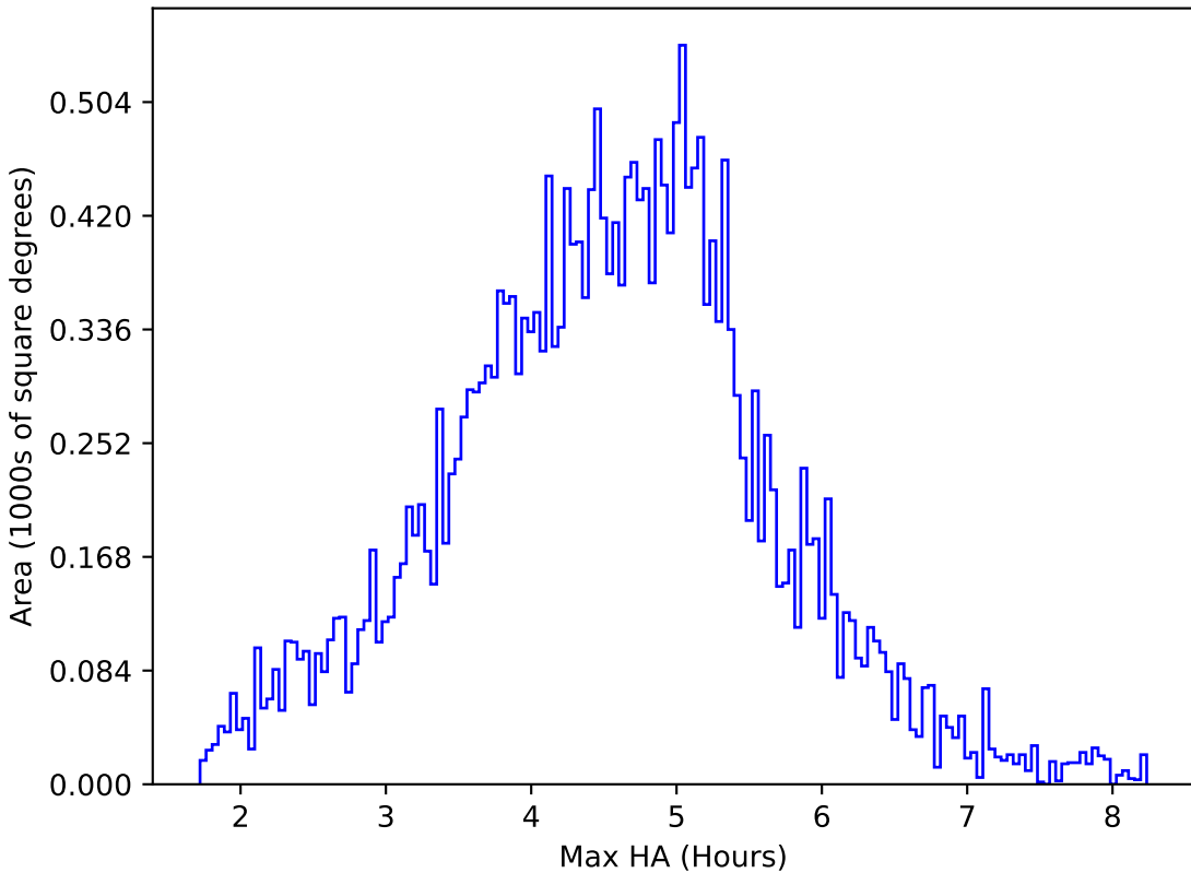
early_u_fpextra2.0_v3.4_10yrs All sky i band: Max HA
