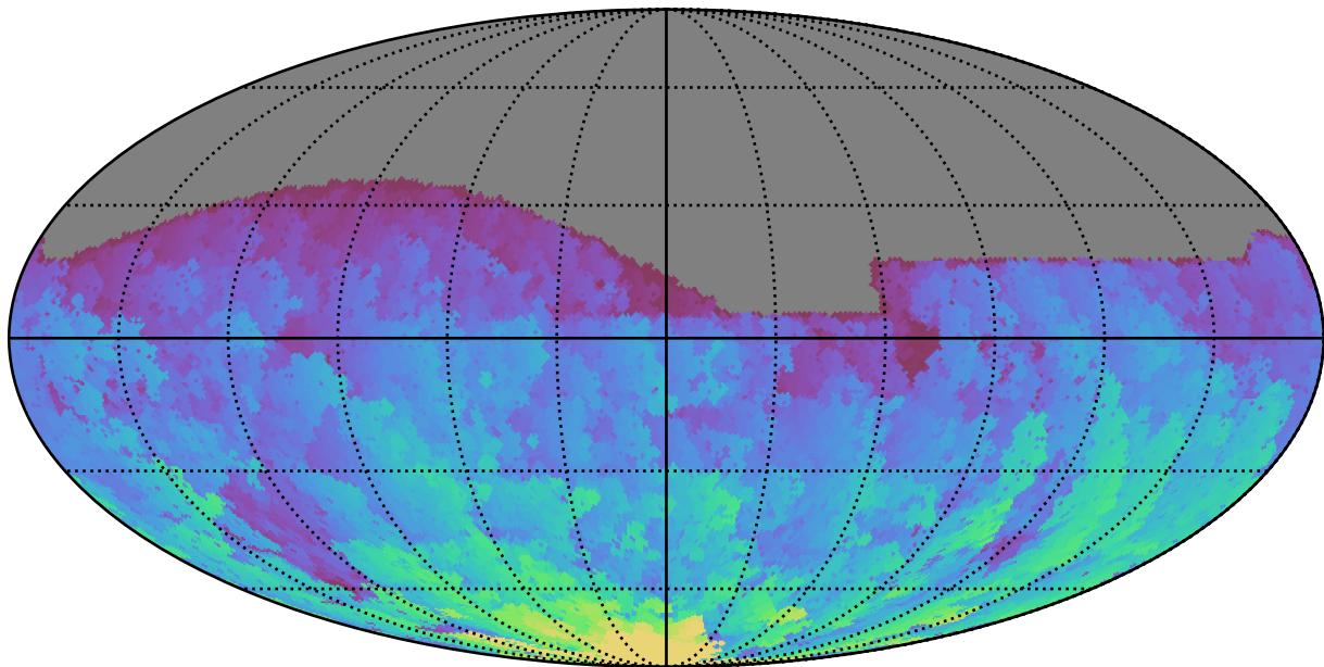
early_u_fpextra2.0_v3.4_10yrs All sky g band: Max HA
