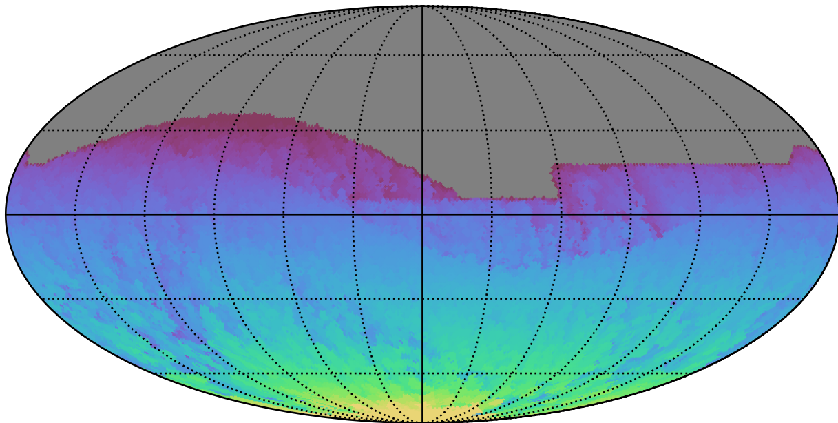
early_u_fpextra2.0_v3.4_10yrs All sky all bands: Max HA
