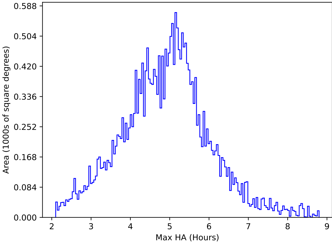
early_u_fpextra2.0_v3.4_10yrs All sky all bands: Max HA
