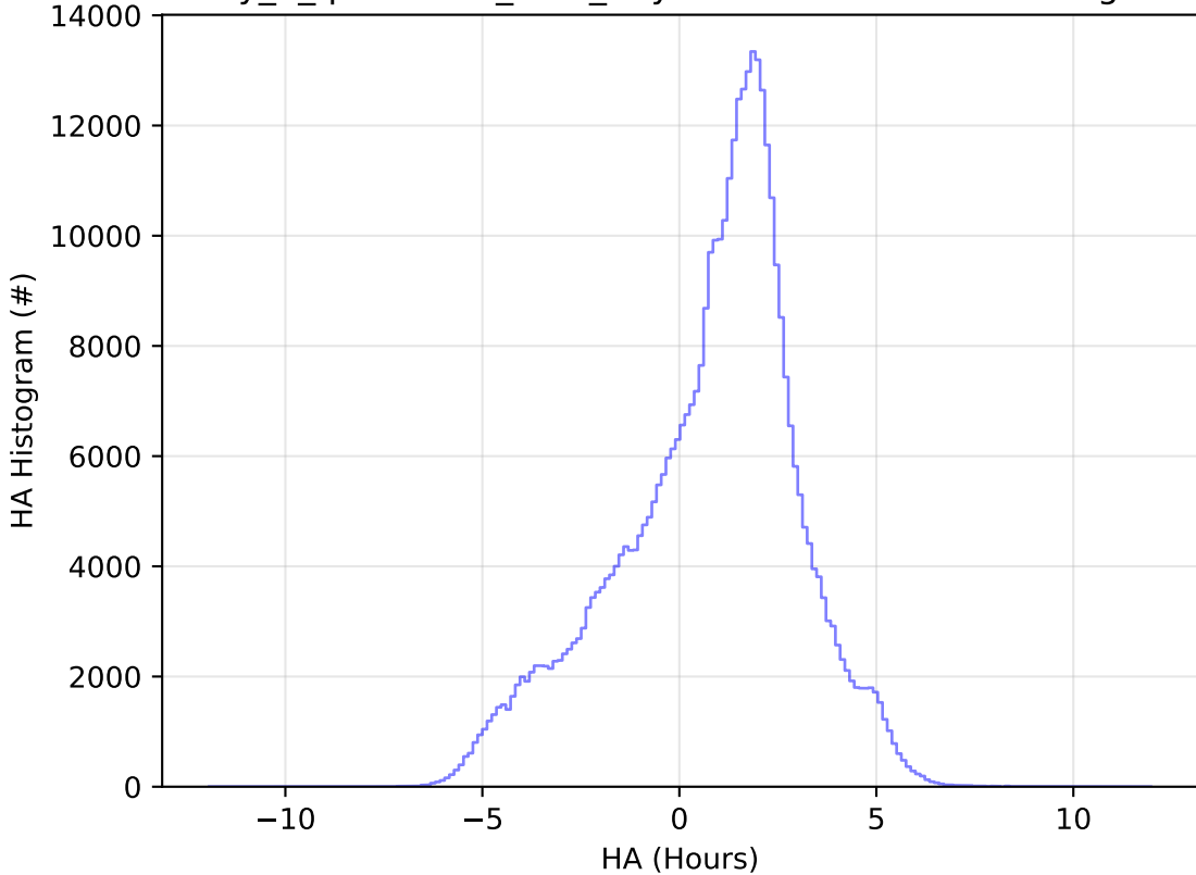
early_u_fpextra2.0_v3.4_10yrs WFD z band: HA Histogram
