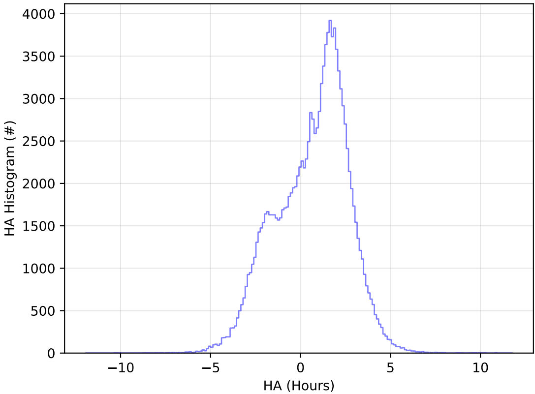
early_u_fpextra2.0_v3.4_10yrs WFD u band: HA Histogram
