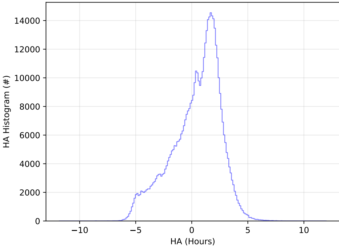
early_u_fpextra2.0_v3.4_10yrs WFD r band: HA Histogram
