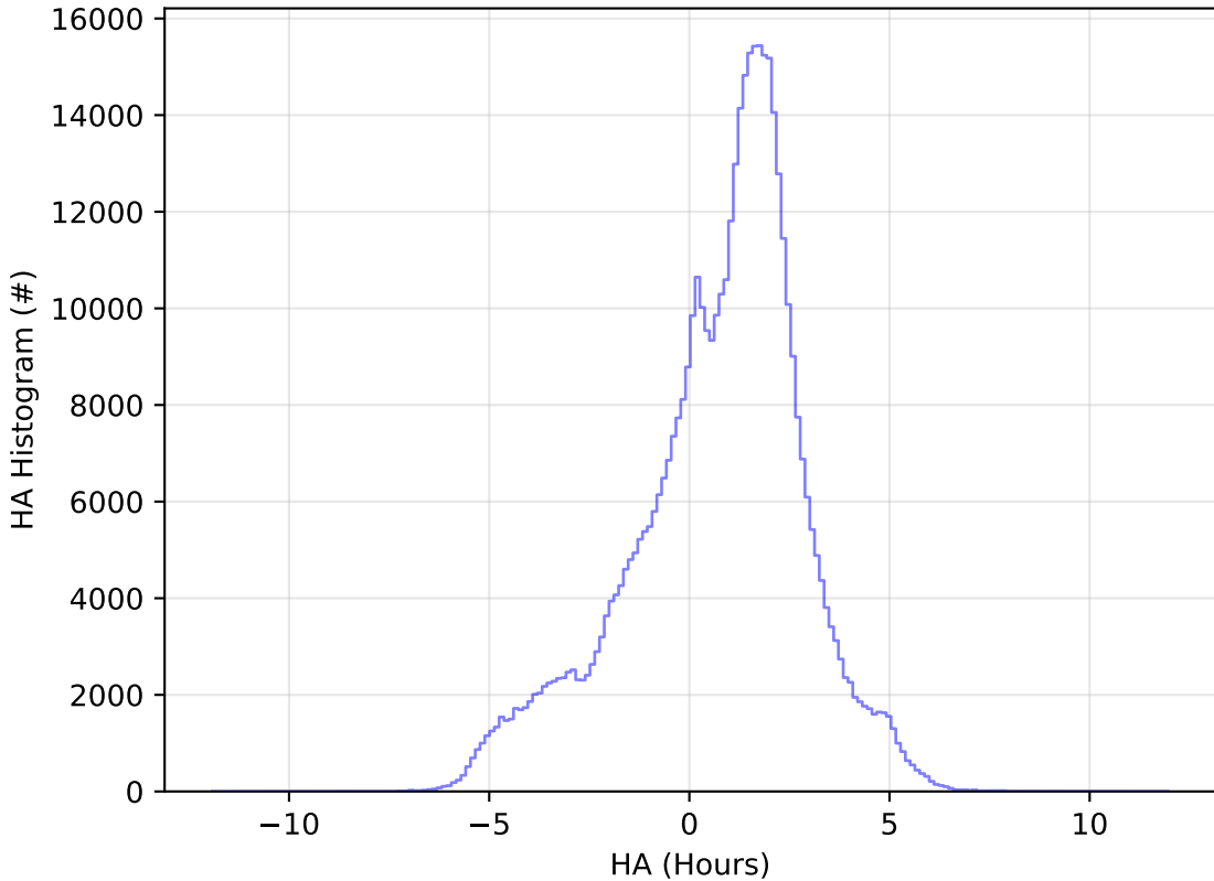
early_u_fpextra2.0_v3.4_10yrs WFD i band: HA Histogram
