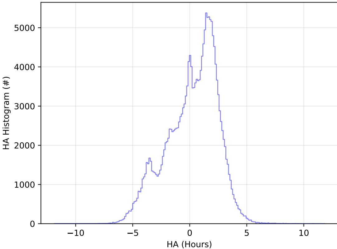
early_u_fpextra2.0_v3.4_10yrs WFD g band: HA Histogram
