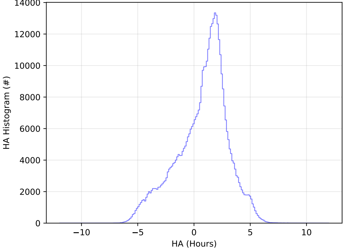
early_u_fpextra2.0_v3.4_10yrs All sky z band: HA Histogram
