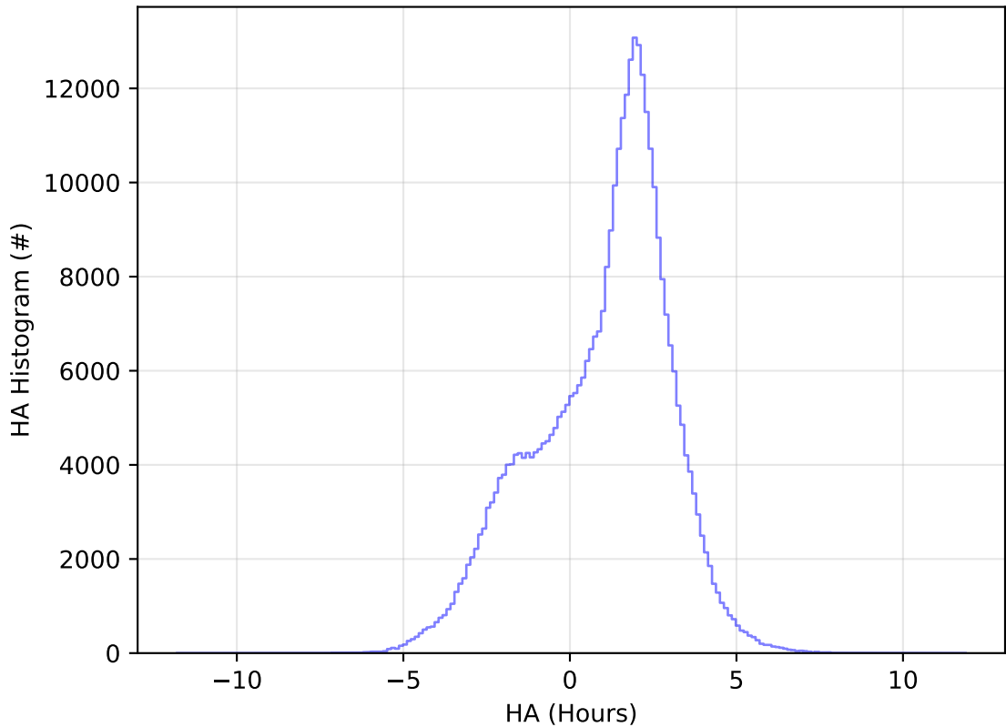
early_u_fpextra2.0_v3.4_10yrs All sky y band: HA Histogram
